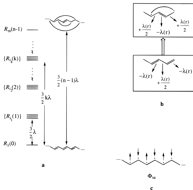
SCHEME 1: (a) Spectrum of the Rumer Basis Set for n -Electron Pairs. (b) Schematic Representation of the Elementary Excitation of the Electron Pairs, and Energy Terms for a Paired Bond and a Couple of Nonbonded Electrons (c) Spin Alternant Determinant (spins shown by arrows)
